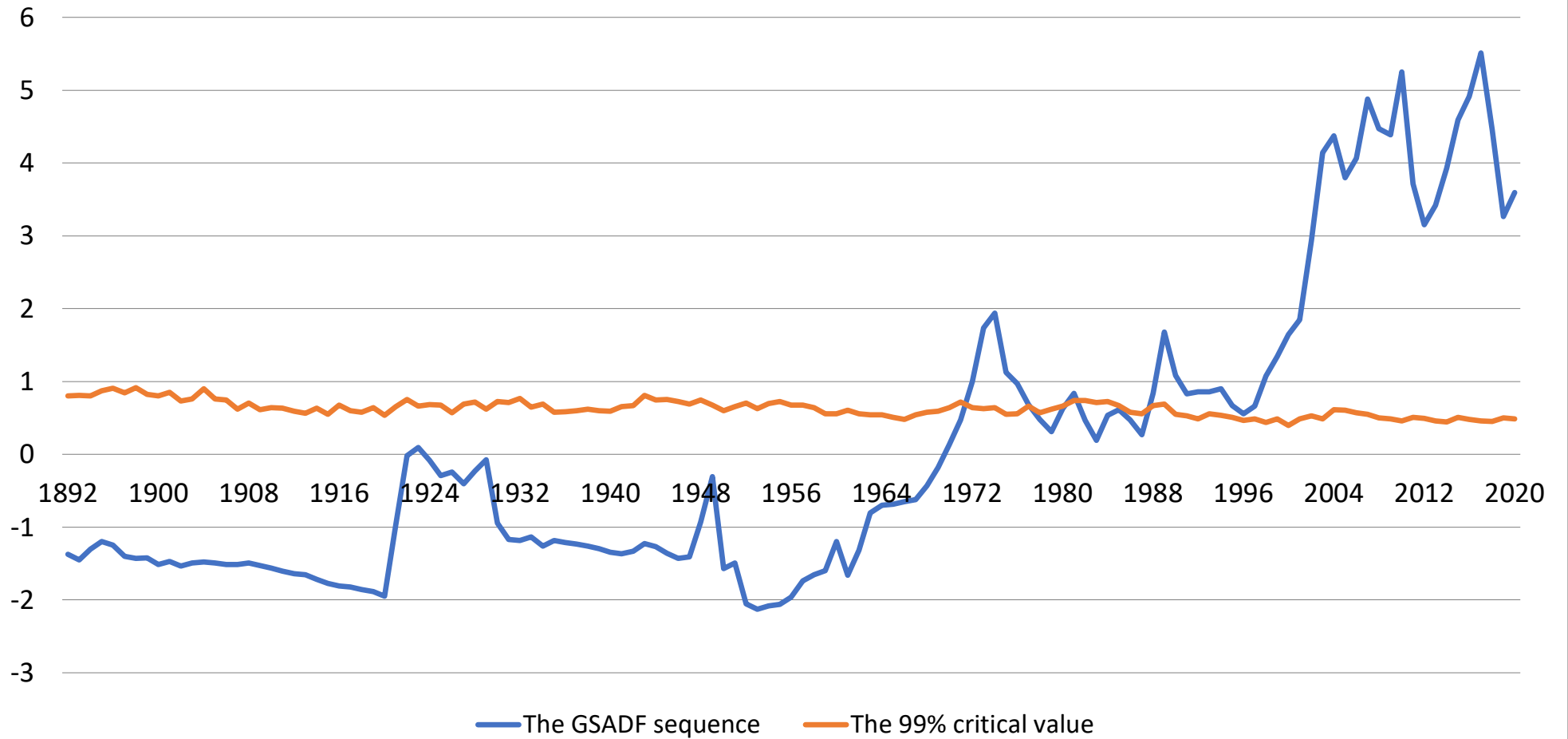
Figure 3 Date-stamping bubble periods in the Australian real house prices: The GSADF test
